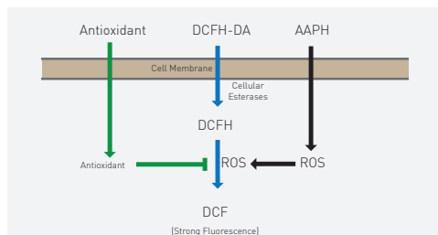
Fig. 1: Principle of the OxiSelect Cellular Antioxidant Assay.
