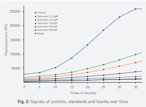
Fig. 2: Signals of controls, standards and blanks over time.
